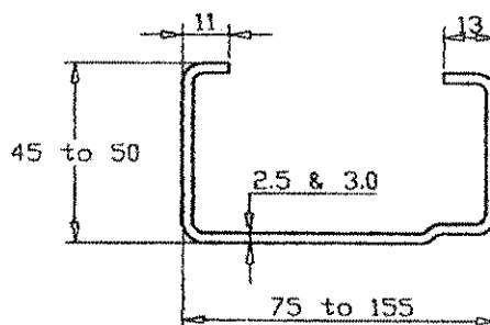
Racking Upright
