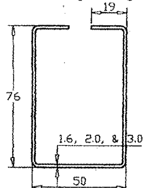
Racking Upright
