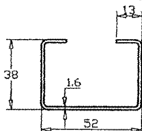
Racking Upright
