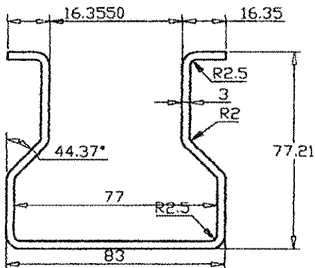
Racking Upright
