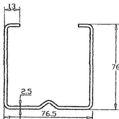
Racking Upright
