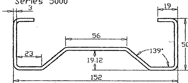
Box Beam
