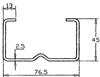
Racking Upright
