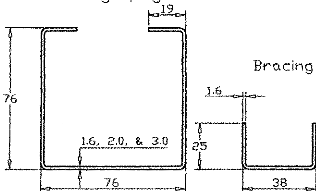
Racking Upright
