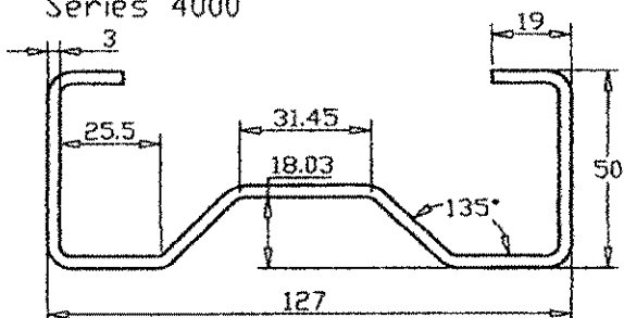
Racking Upright
